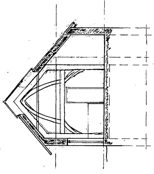
SECTION
